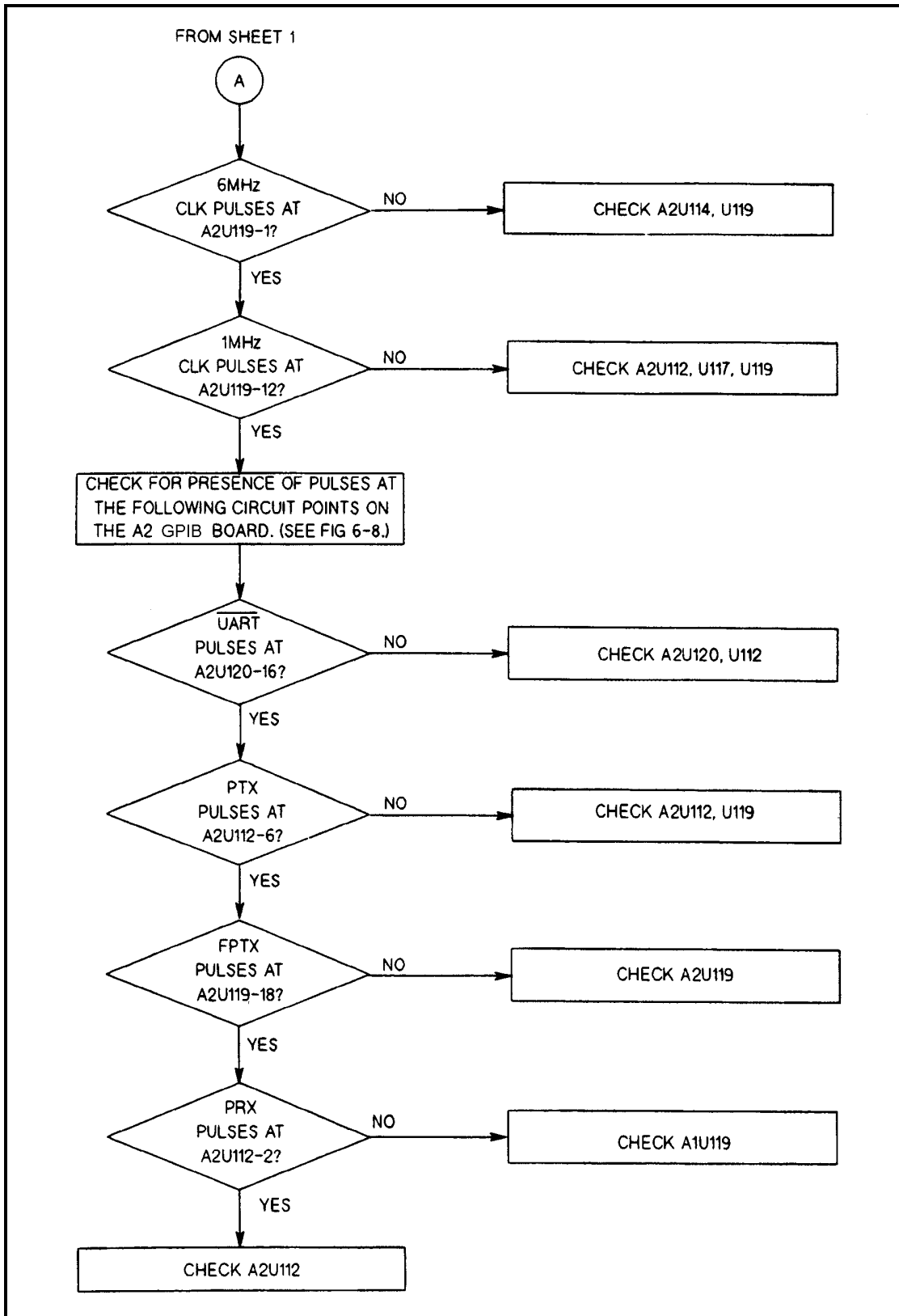
Figure 3-10. Serial Down Troubleshooting (Sheet 2 of 2)
